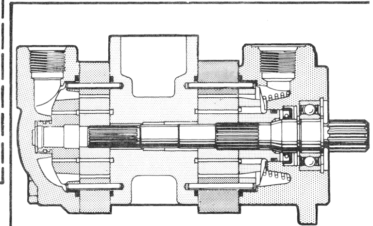
ASSEMBLY VIEW
