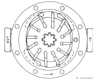
ASSEMBLED VIEW FACING HEAD END
