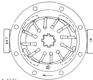
ASSEMBLED VIEW FACING HEAD END
