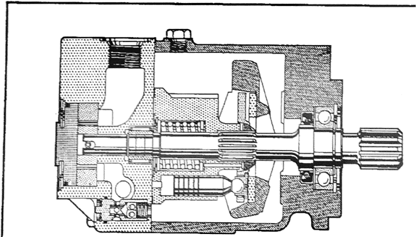
ASSEMBLY VIEW
