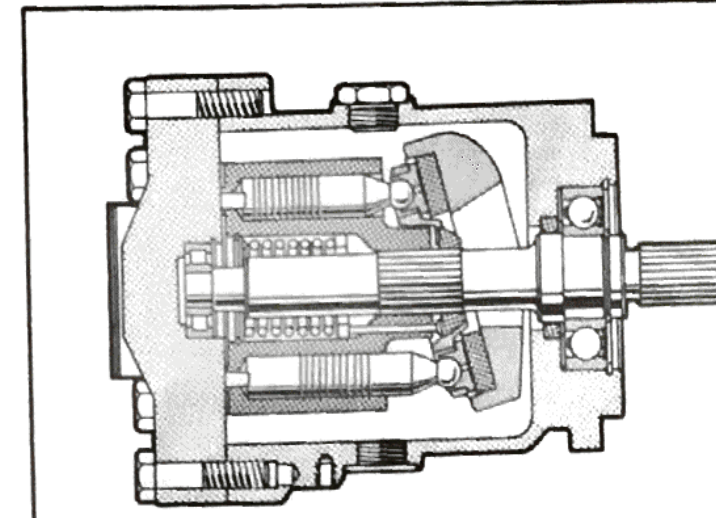
ASSEMBLY VIEW
