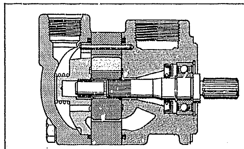
ASSEMBLY VIEW
